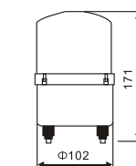
OUTER SIZE
